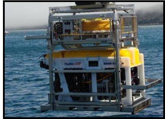
Panther XTP in TMS Cage
